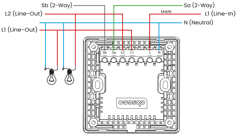
Figure 1: Wiring Diagram – 1-Way Installation
